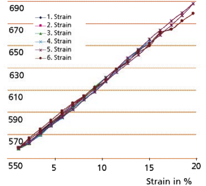
Change in capacitance of the strain sensor
