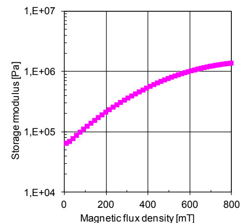
Increase of storage modulus of MRE with magnetic flux density
