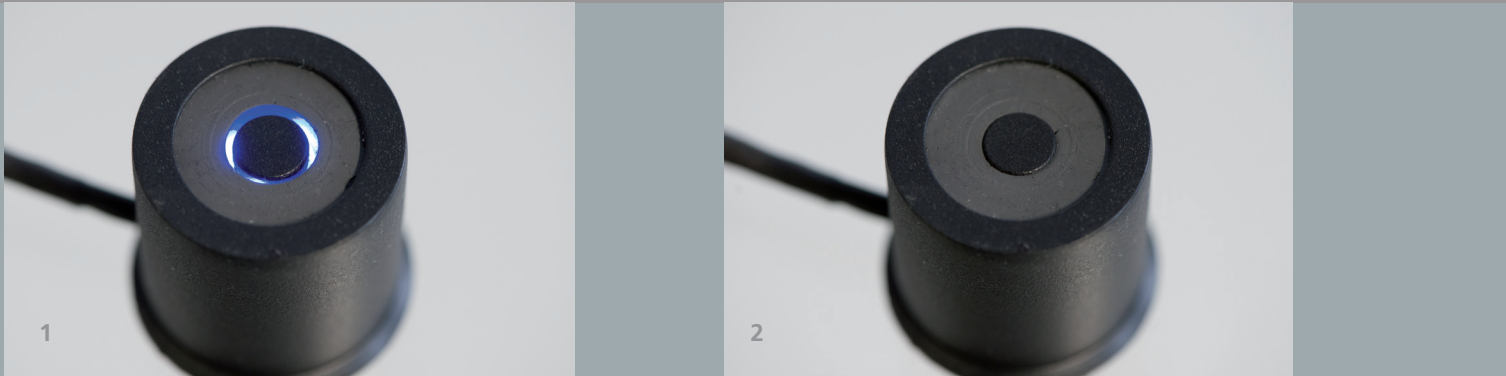
Magnetorheological Elastomer (MRE) disc on a solenoid MRE-valve in the opened 1 and closed 2 state
